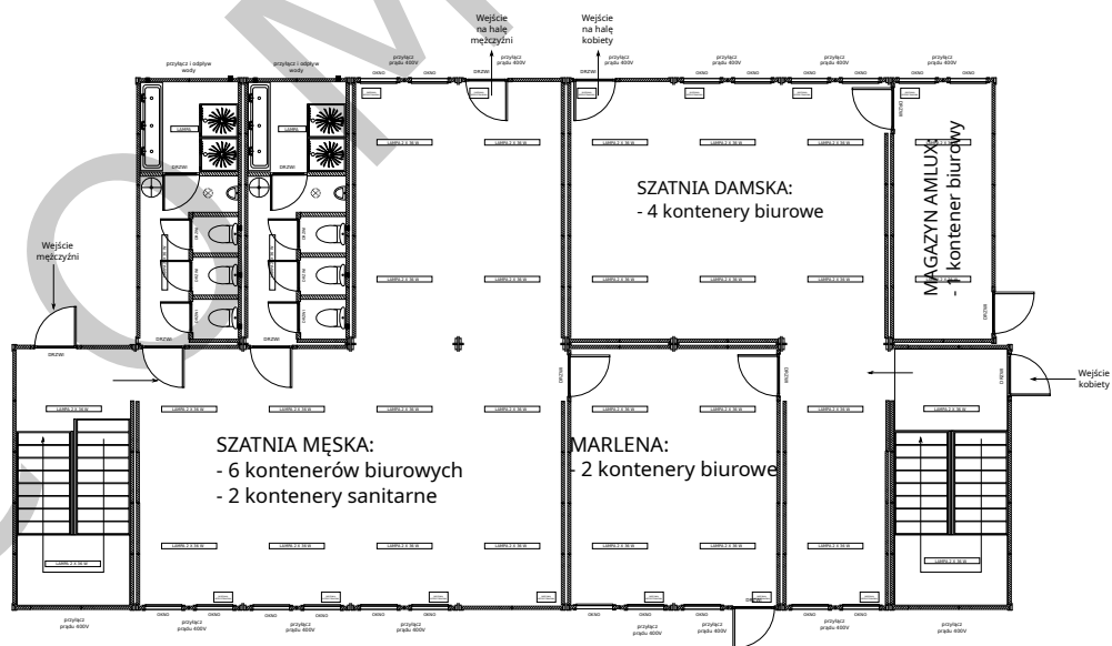
PARTER
